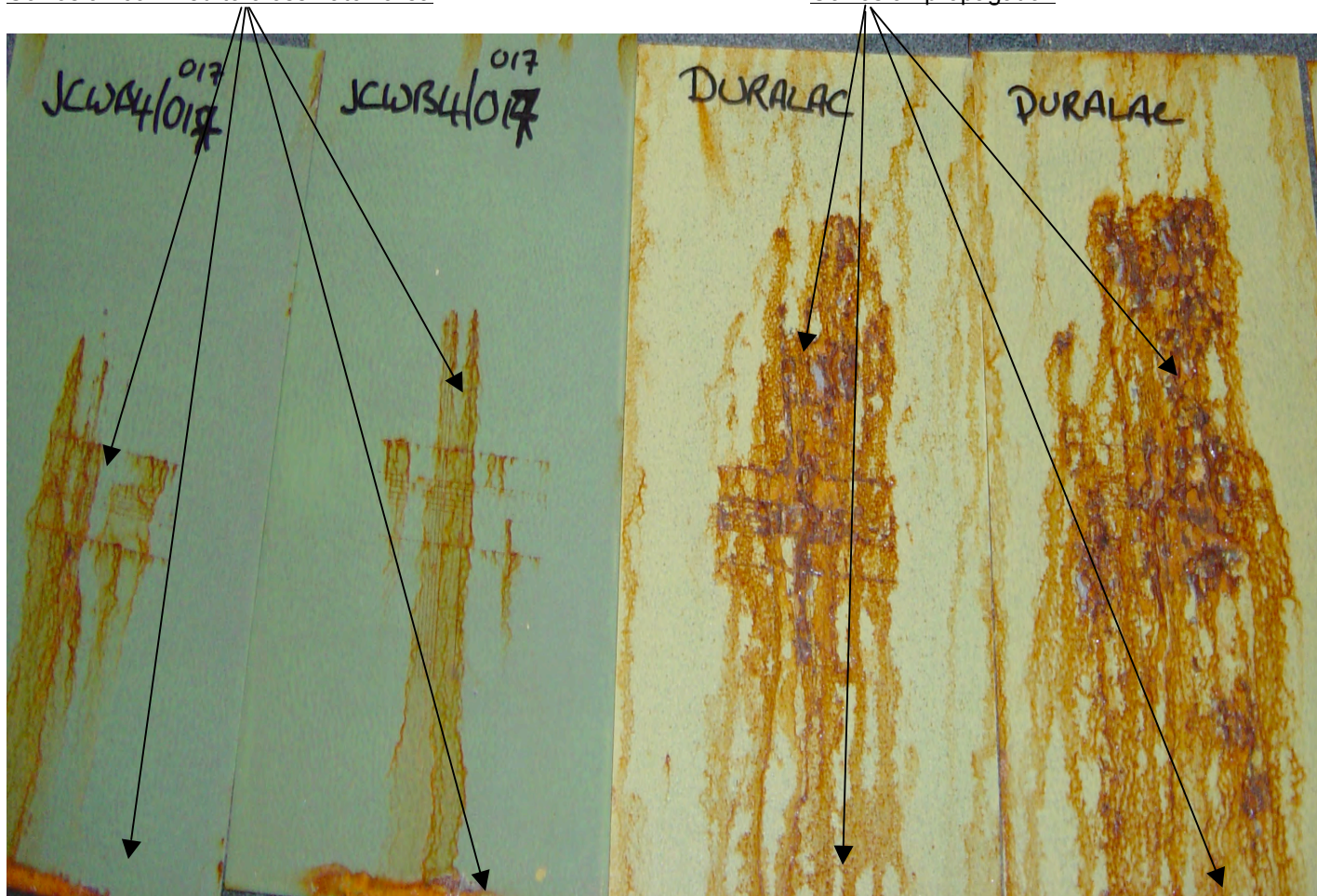
Corrosion confined to cross hatch area
